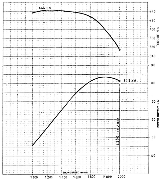
Performance curves
